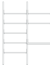
Branch-2 Shelving Unit w/ Desk W64.5 D11.5/20.5 H84 (in) W164 D29/52 H213 (cm)
