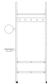
Branch-1 Entryway Unit W48.5 D12.5 H84 (in) W123 D32 H213 (cm)
